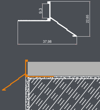
ALÜMİNYUM FAYANS TERAS PROFİLİ Aluminum Tile Terrace Profile
