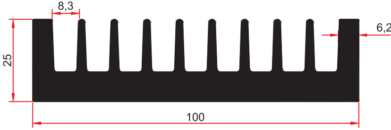
5530 3.831kg/m
