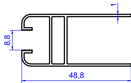
2018 0.436 kg/m
