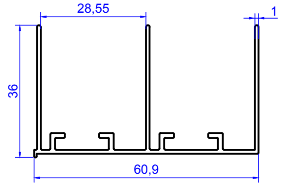
2108 0.558 kg/m
